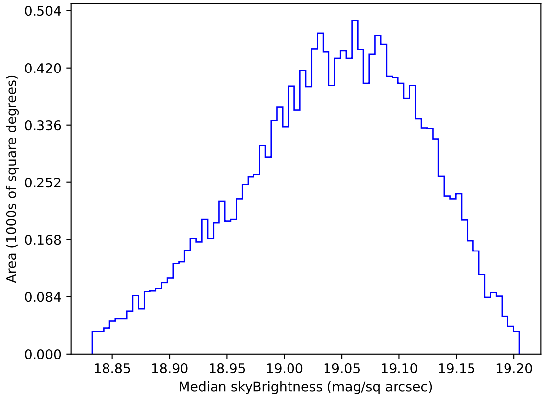
too_elab_heavy_r128_d2_griz_v3.4_10yrs WFD z band: Median skyBrightness
