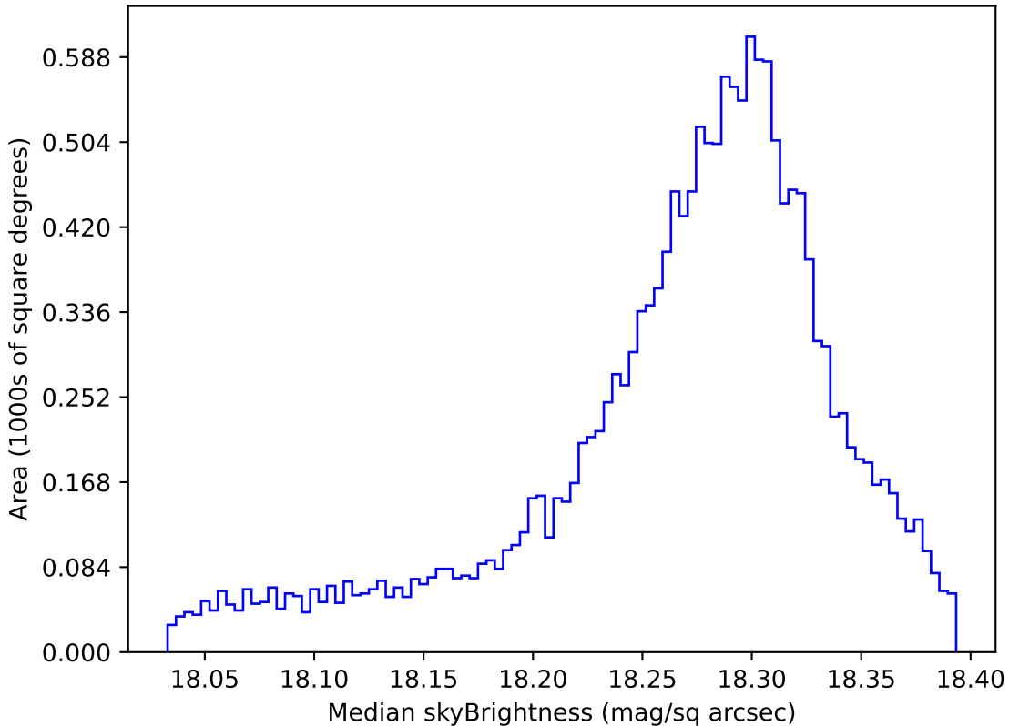
too_elab_heavy_r128_d2_griz_v3.4_10yrs WFD y band: Median skyBrightness
