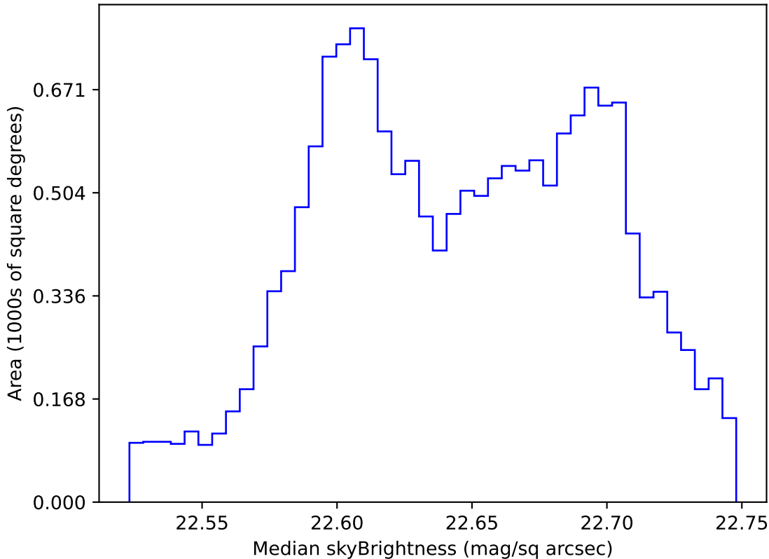
too_elab_heavy_r128_d2_griz_v3.4_10yrs WFD u band: Median skyBrightness
