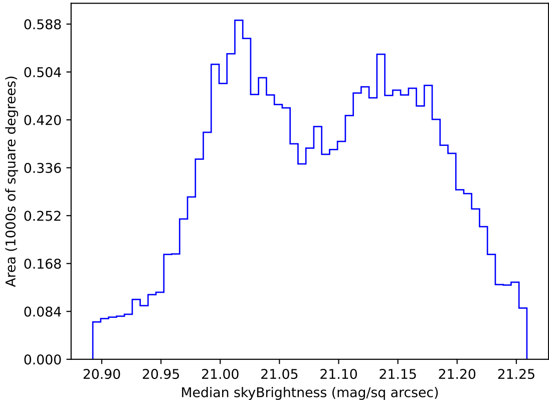
too_elab_heavy_r128_d2_griz_v3.4_10yrs WFD r band: Median skyBrightness
