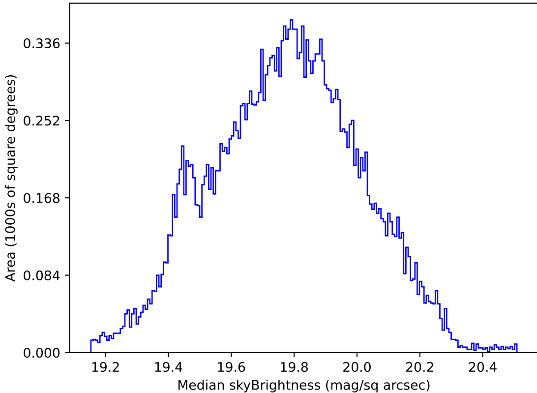
too_elab_heavy_r128_d2_griz_v3.4_10yrs All sky all bands: Median skyBrightness
