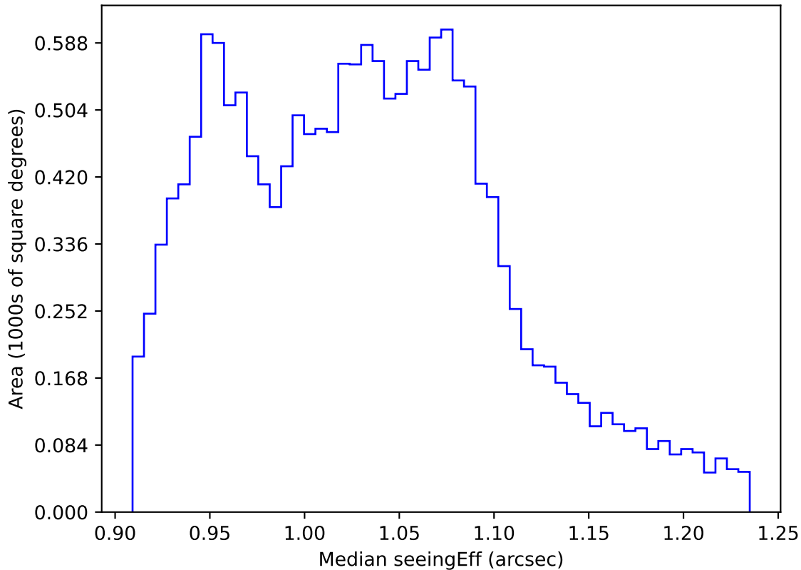
too_elab_heavy_r128_d2_griz_v3.4_10yrs WFD all bands: Median seeingEff
