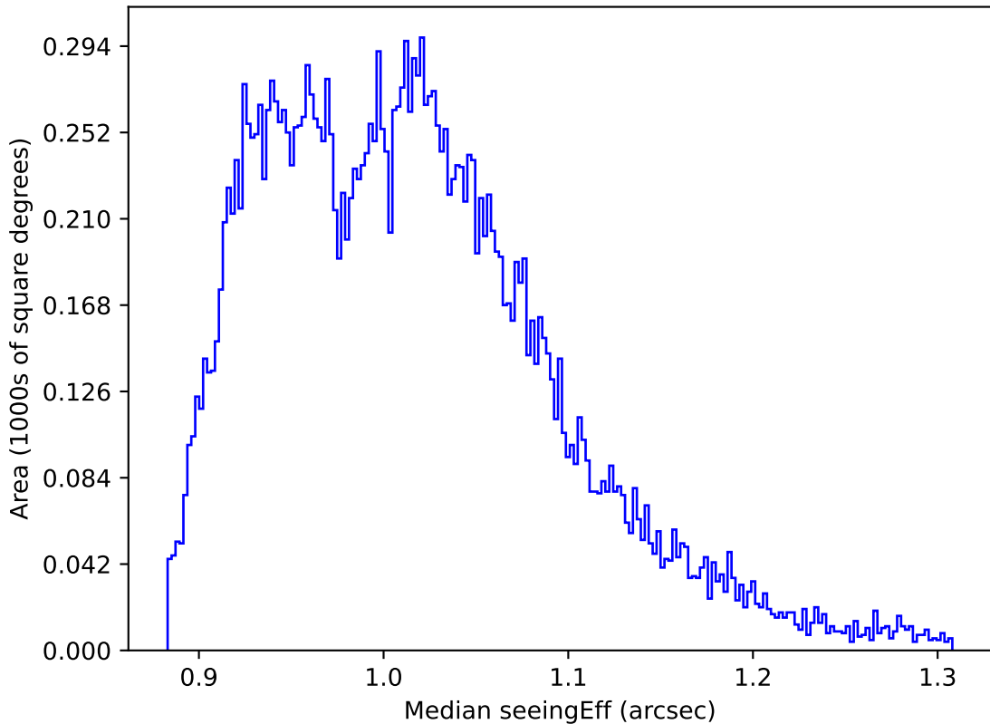
too_elab_heavy_r128_d2_griz_v3.4_10yrs All sky y band: Median seeingEff
