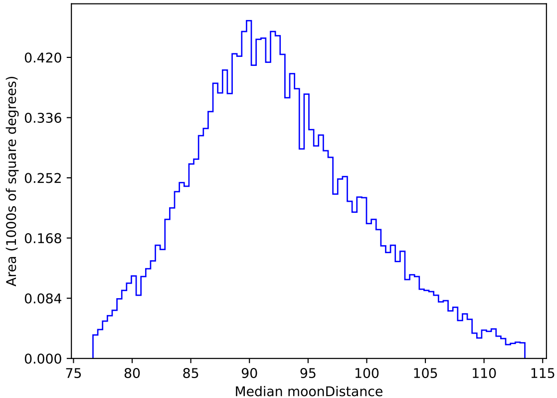
too_elab_heavy_r128_d2_griz_v3.4_10yrs WFD i band: Median moonDistance
