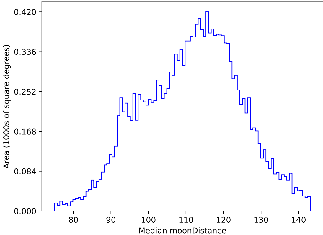
too_elab_heavy_r128_d2_griz_v3.4_10yrs WFD g band: Median moonDistance
