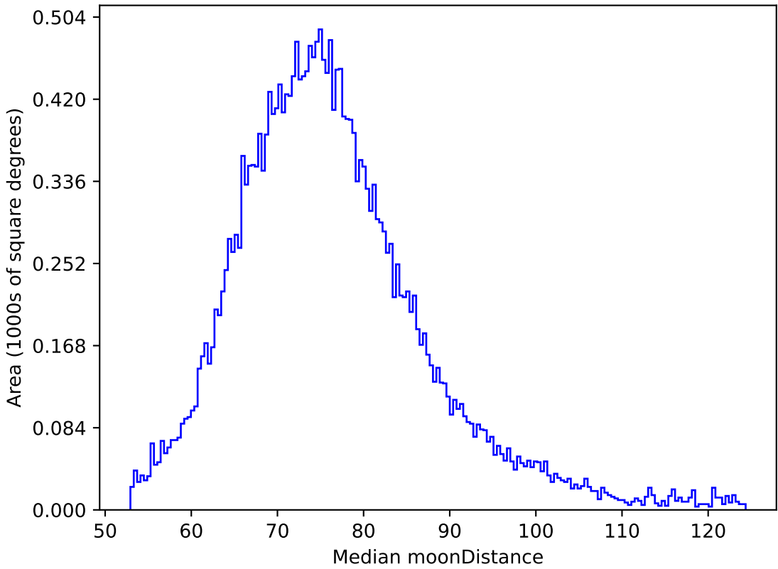
too_elab_heavy_r128_d2_griz_v3.4_10yrs All sky z band: Median moonDistance
