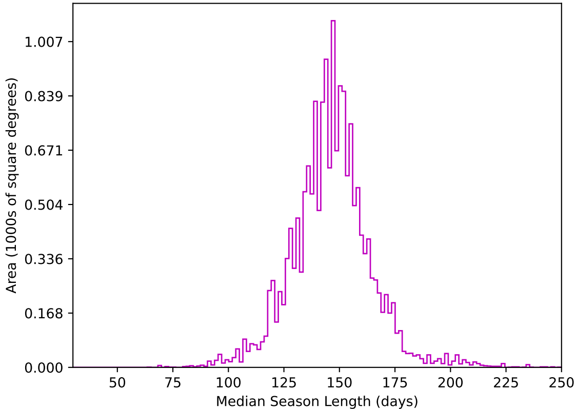
too_elab_heavy_r128_d2_griz_v3.4_10yrs WFD z band: Median Season Length
