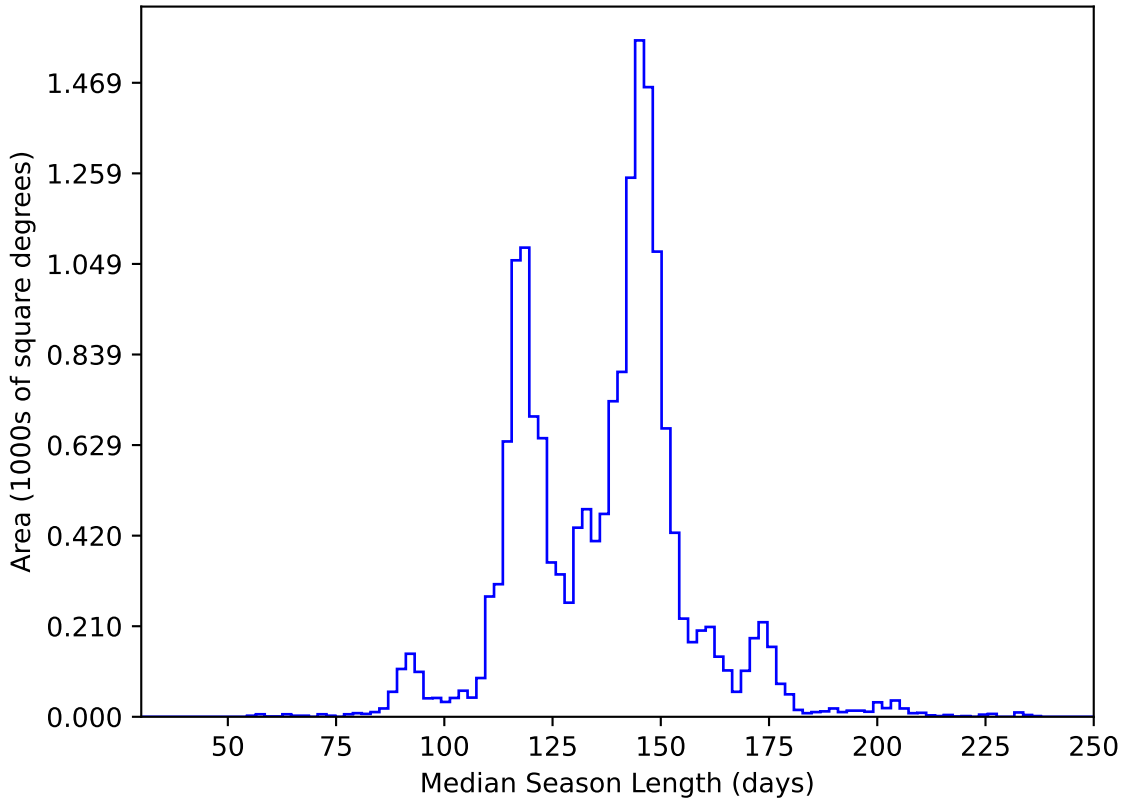
too_elab_heavy_r128_d2_griz_v3.4_10yrs WFD y band: Median Season Length
