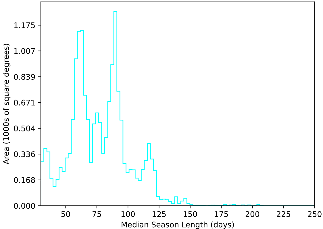
too_elab_heavy_r128_d2_griz_v3.4_10yrs WFD u band: Median Season Length
