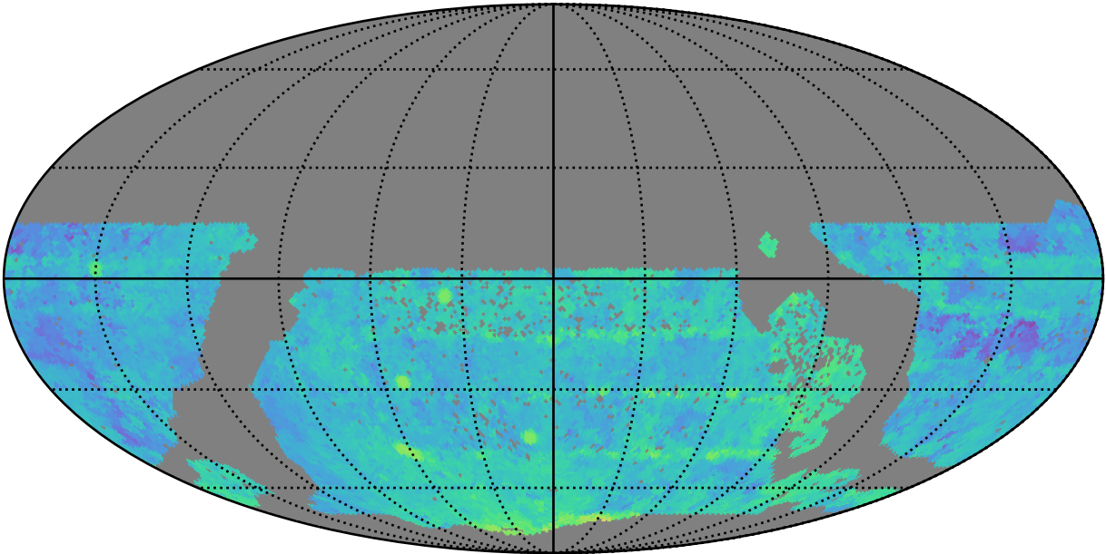
too_elab_heavy_r128_d2_griz_v3.4_10yrs WFD i band: Median Season Length
