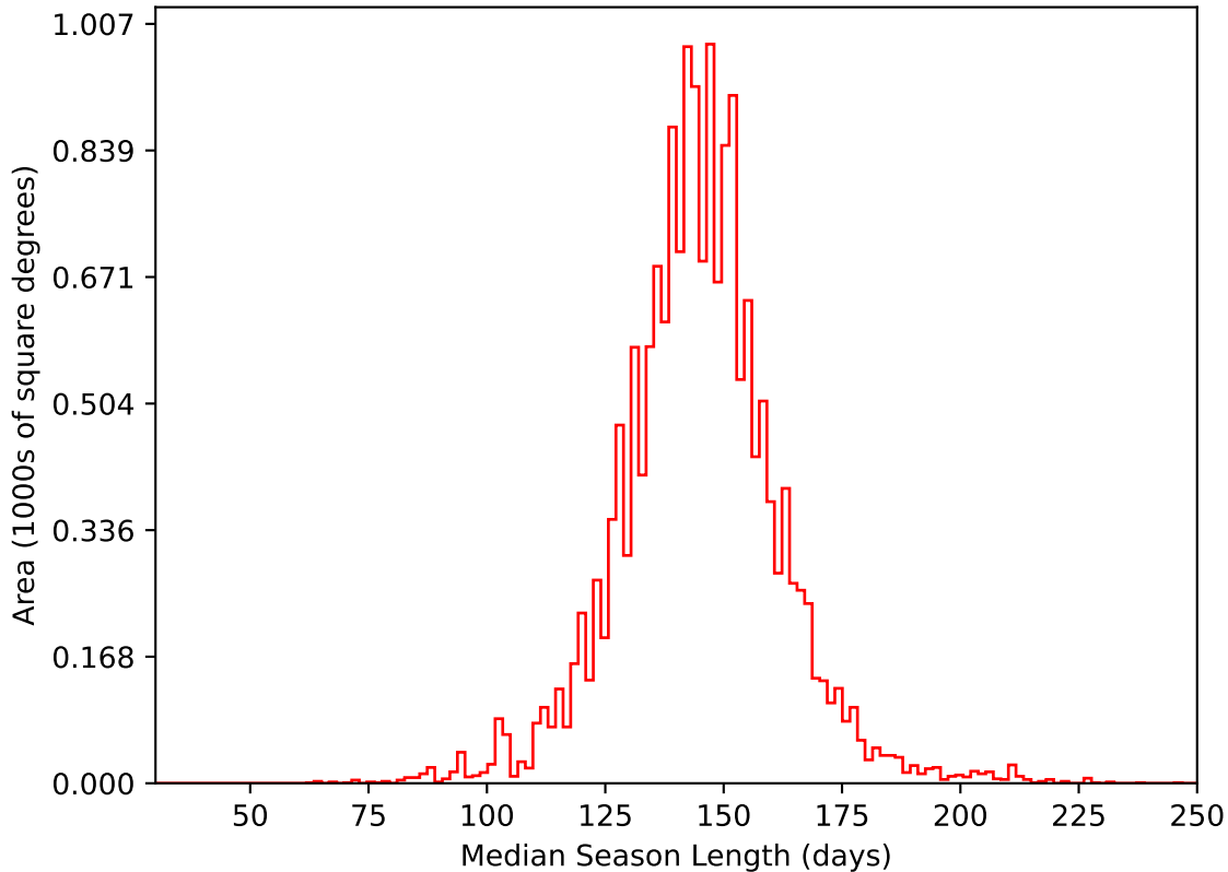
too_elab_heavy_r128_d2_griz_v3.4_10yrs WFD i band: Median Season Length
