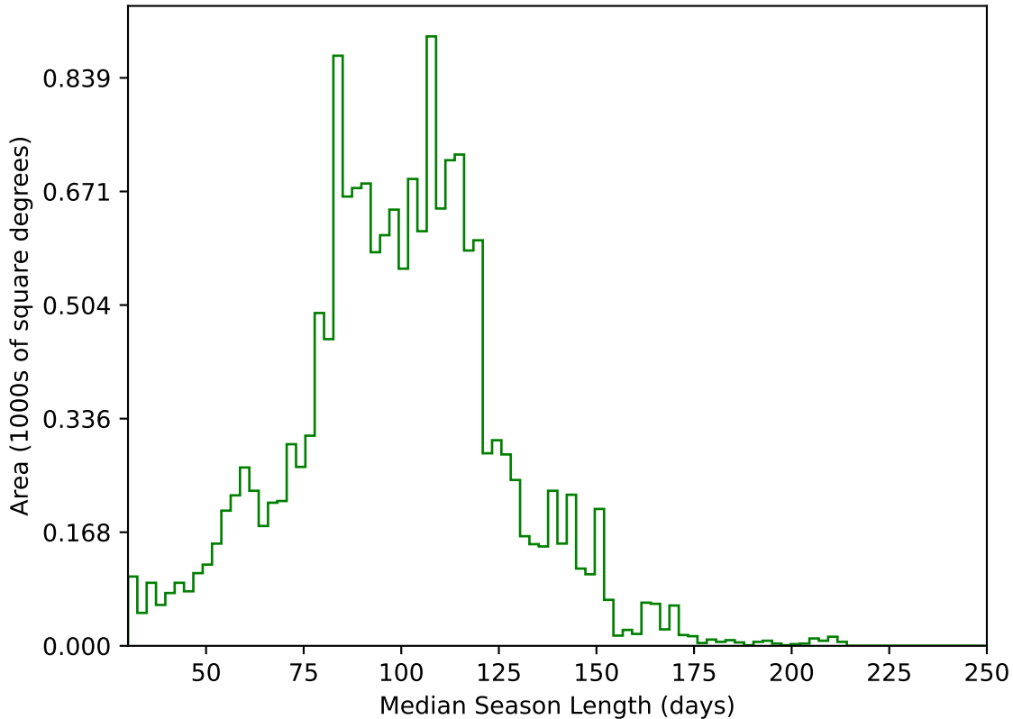
too_elab_heavy_r128_d2_griz_v3.4_10yrs WFD g band: Median Season Length
