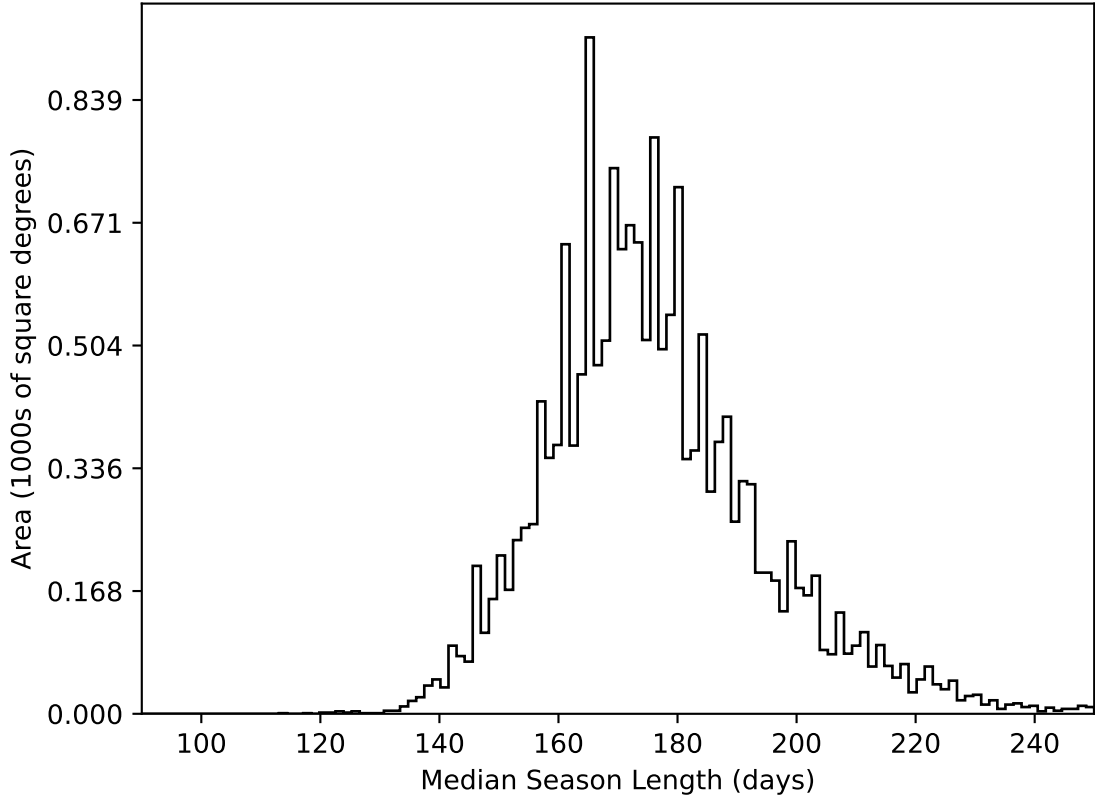
too_elab_heavy_r128_d2_griz_v3.4_10yrs WFD all bands: Median Season Length
