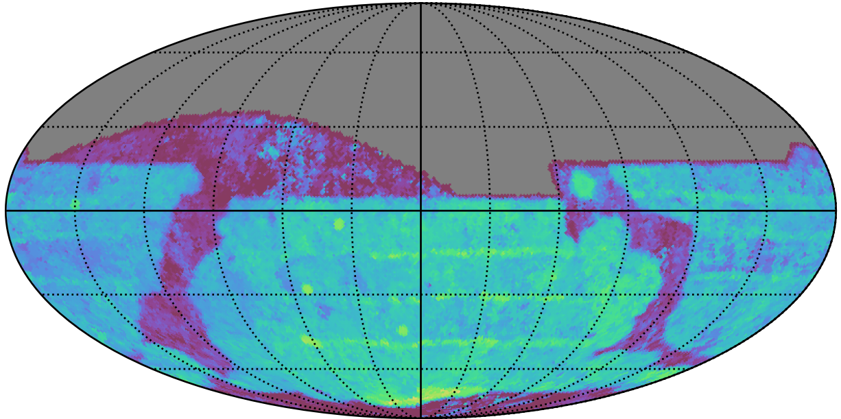
too_elab_heavy_r128_d2_griz_v3.4_10yrs All sky z band: Median Season Length
