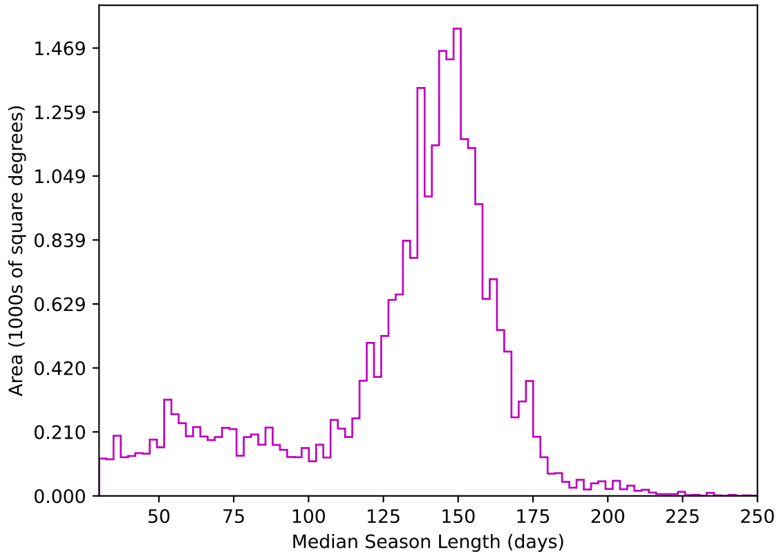
too_elab_heavy_r128_d2_griz_v3.4_10yrs All sky z band: Median Season Length
