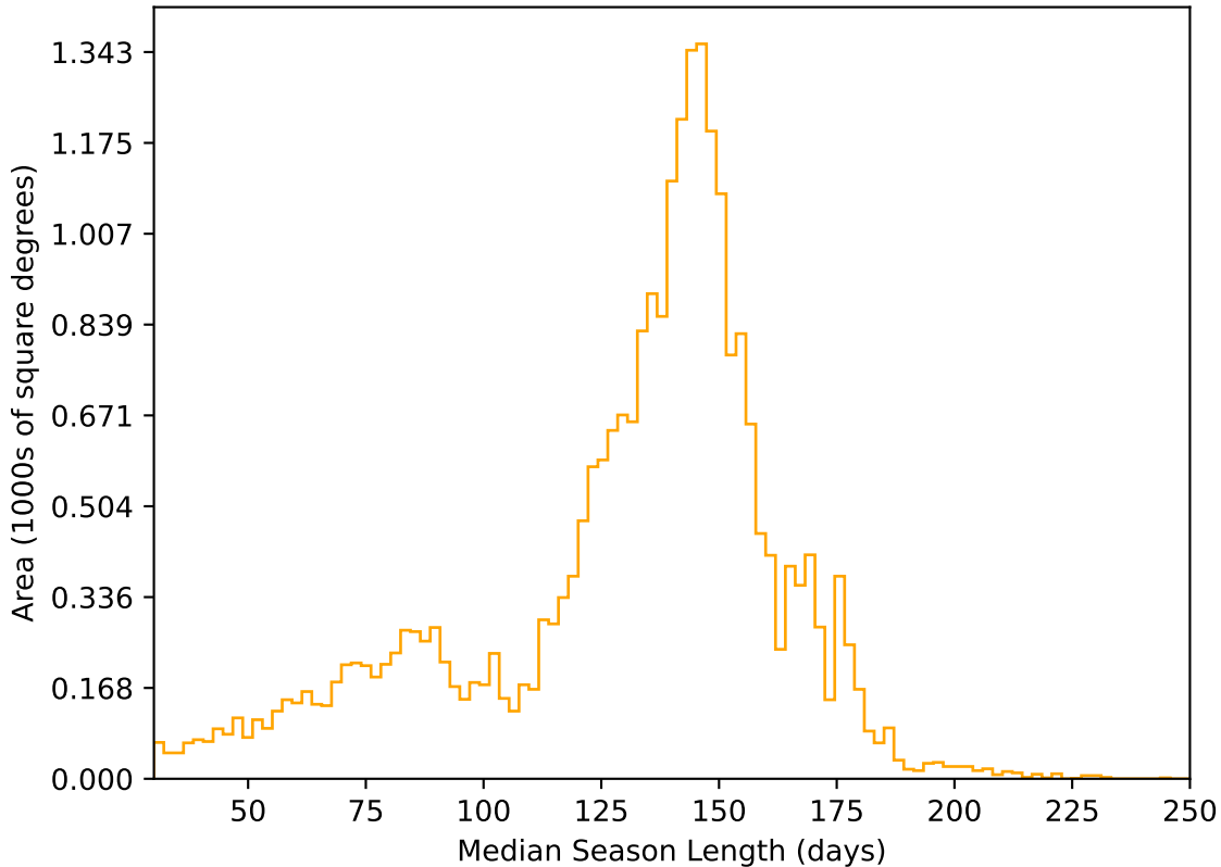
too_elab_heavy_r128_d2_griz_v3.4_10yrs All sky r band: Median Season Length
