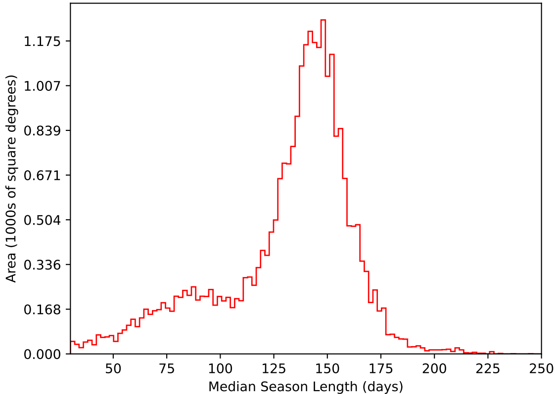
too_elab_heavy_r128_d2_griz_v3.4_10yrs All sky i band: Median Season Length
