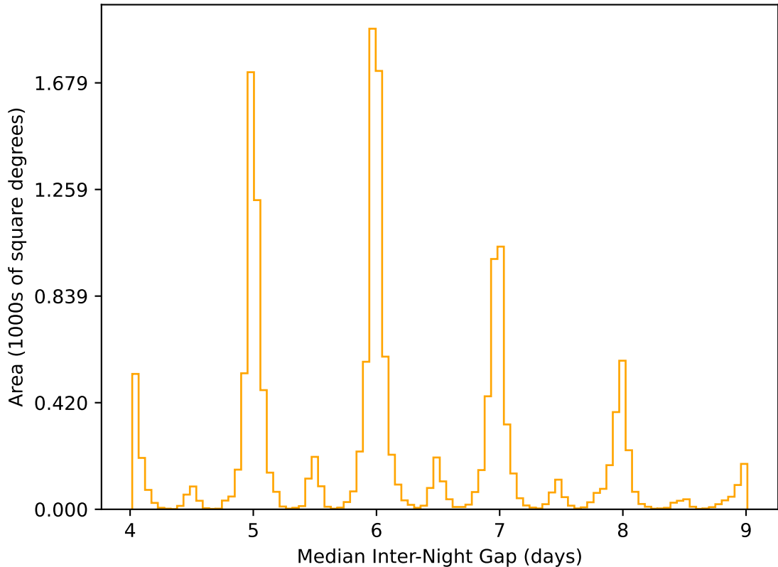
too_elab_heavy_r128_d2_griz_v3.4_10yrs WFD r band: Median Inter-Night Gap
