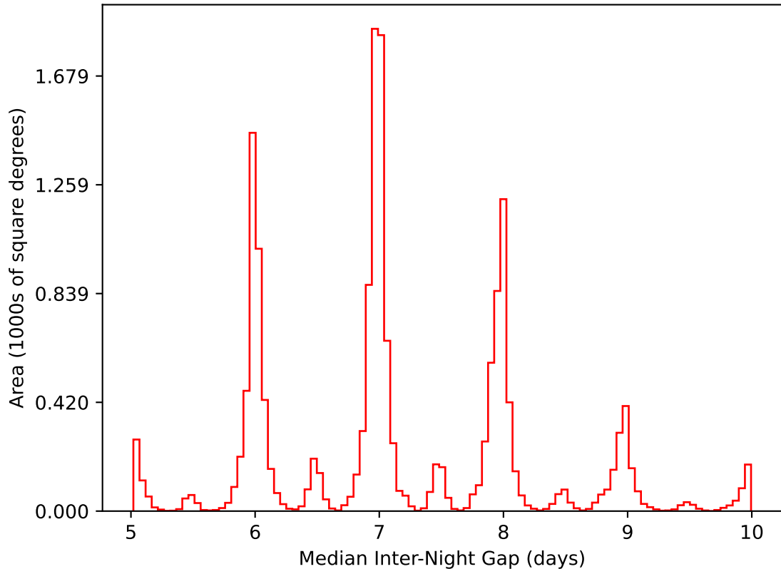
too_elab_heavy_r128_d2_griz_v3.4_10yrs WFD i band: Median Inter-Night Gap
