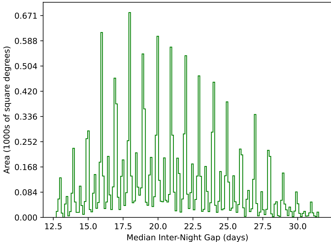
too_elab_heavy_r128_d2_griz_v3.4_10yrs WFD g band: Median Inter-Night Gap
