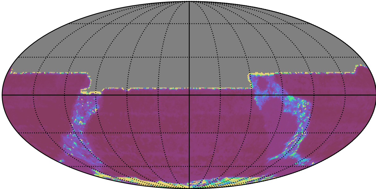
too_elab_heavy_r128_d2_griz_v3.4_10yrs All sky y band: Median Inter-Night Gap
