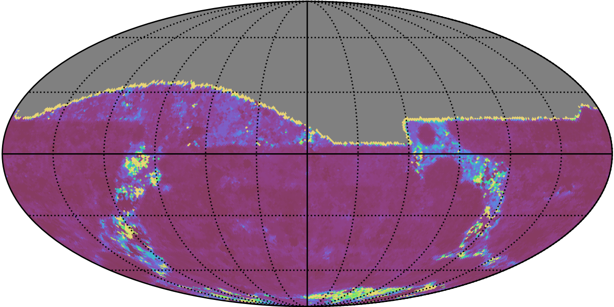
too_elab_heavy_r128_d2_griz_v3.4_10yrs All sky g band: Median Inter-Night Gap
