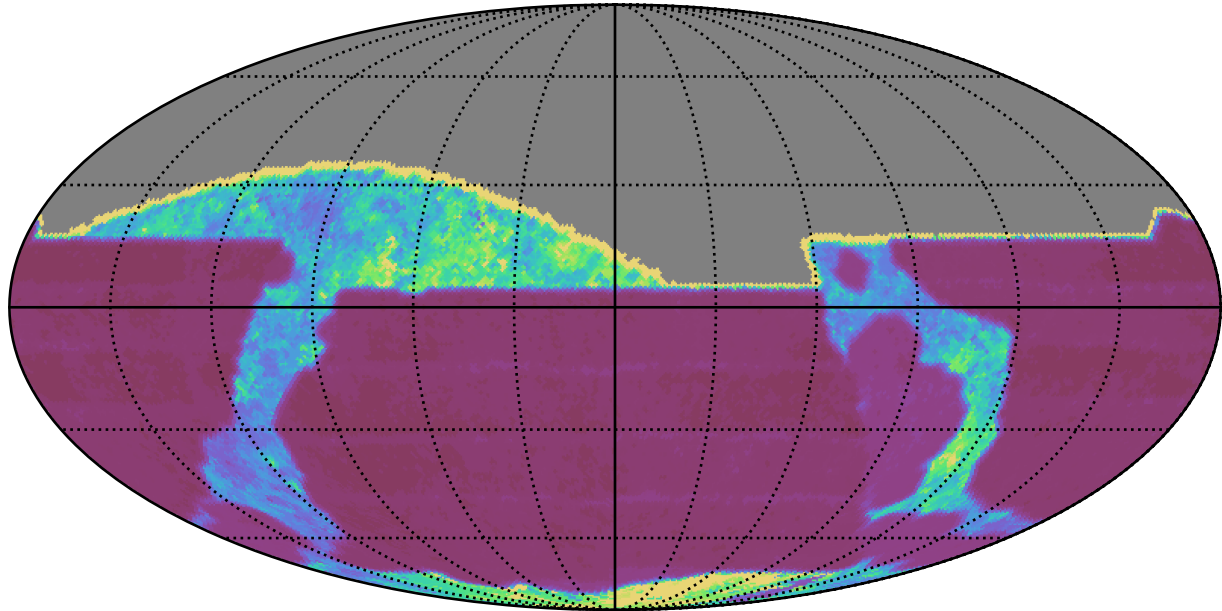
too_elab_heavy_r128_d2_griz_v3.4_10yrs All sky all bands: Median Inter-Night Gap
