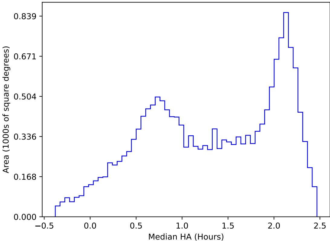
too_elab_heavy_r128_d2_griz_v3.4_10yrs WFD y band: Median HA
