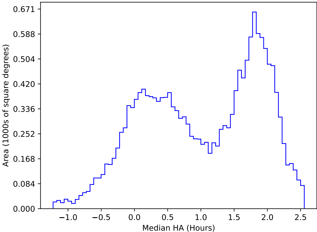
too_elab_heavy_r128_d2_griz_v3.4_10yrs WFD u band: Median HA
