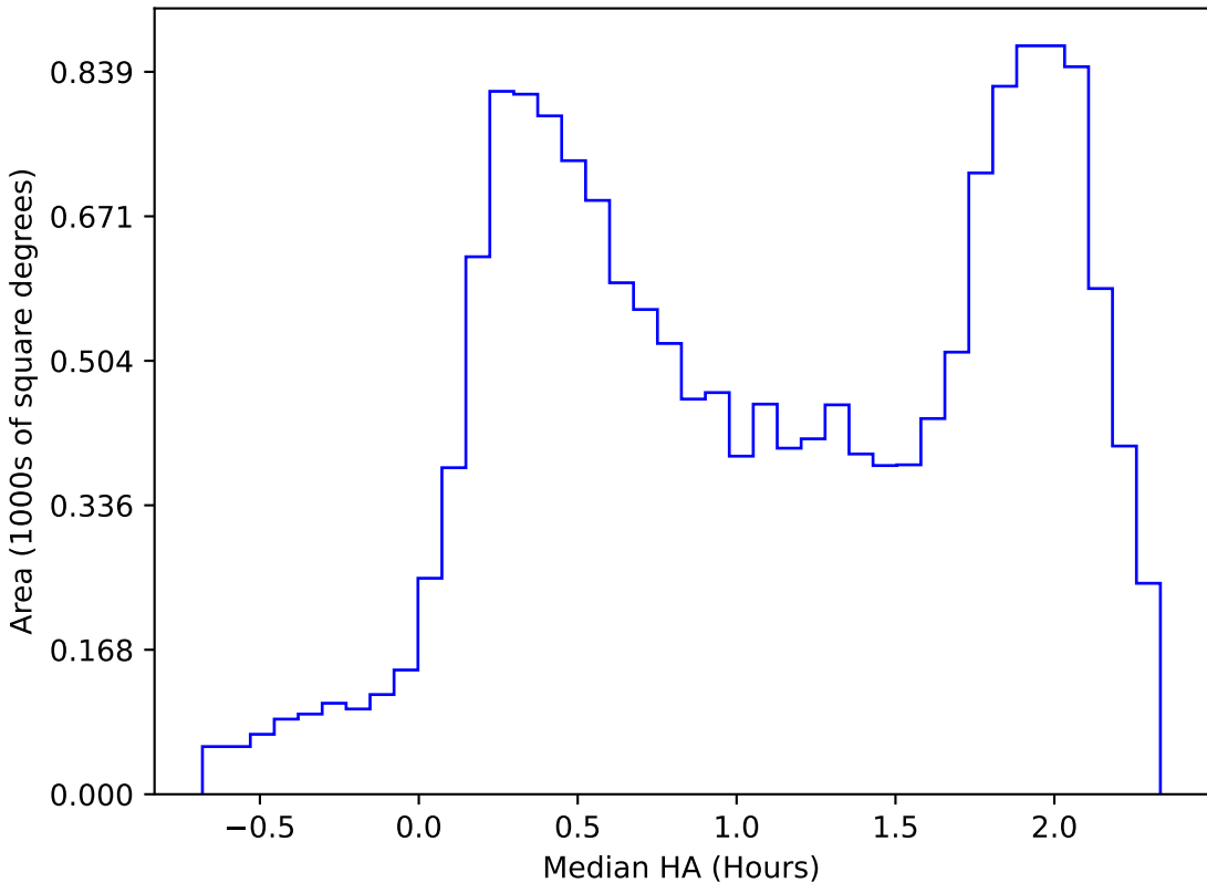
too_elab_heavy_r128_d2_griz_v3.4_10yrs WFD i band: Median HA
