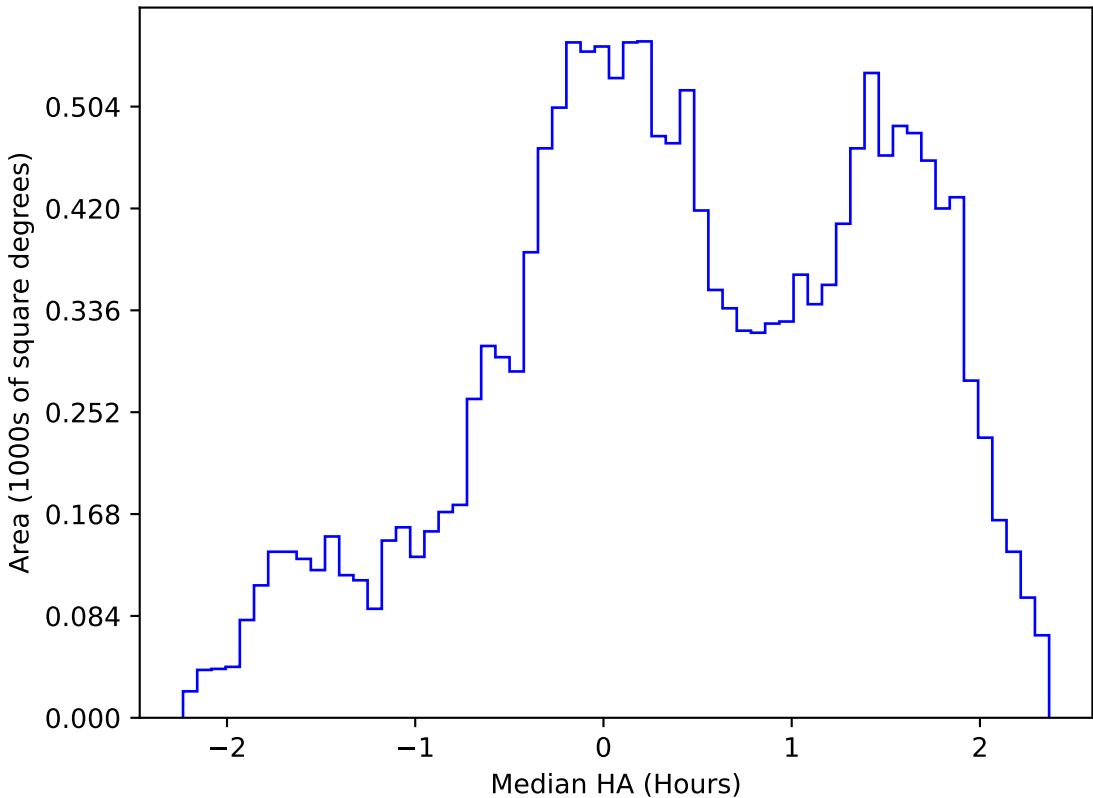
too_elab_heavy_r128_d2_griz_v3.4_10yrs WFD g band: Median HA
