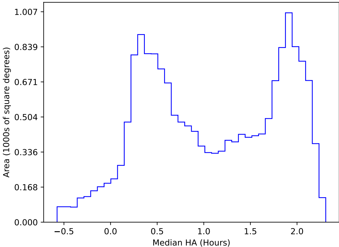
too_elab_heavy_r128_d2_griz_v3.4_10yrs WFD all bands: Median HA
