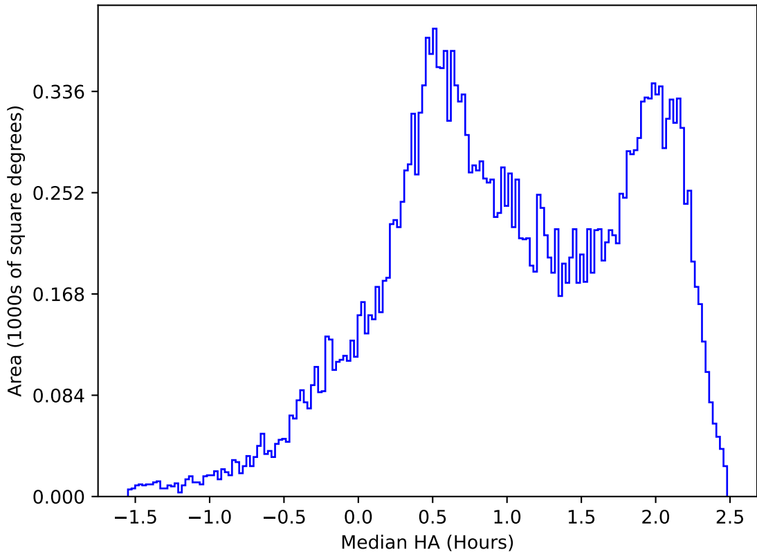
too_elab_heavy_r128_d2_griz_v3.4_10yrs All sky z band: Median HA
