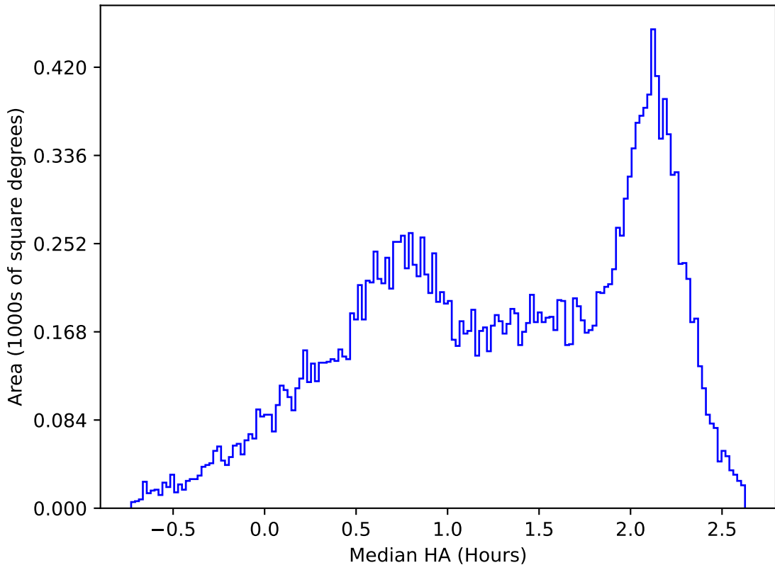
too_elab_heavy_r128_d2_griz_v3.4_10yrs All sky y band: Median HA
