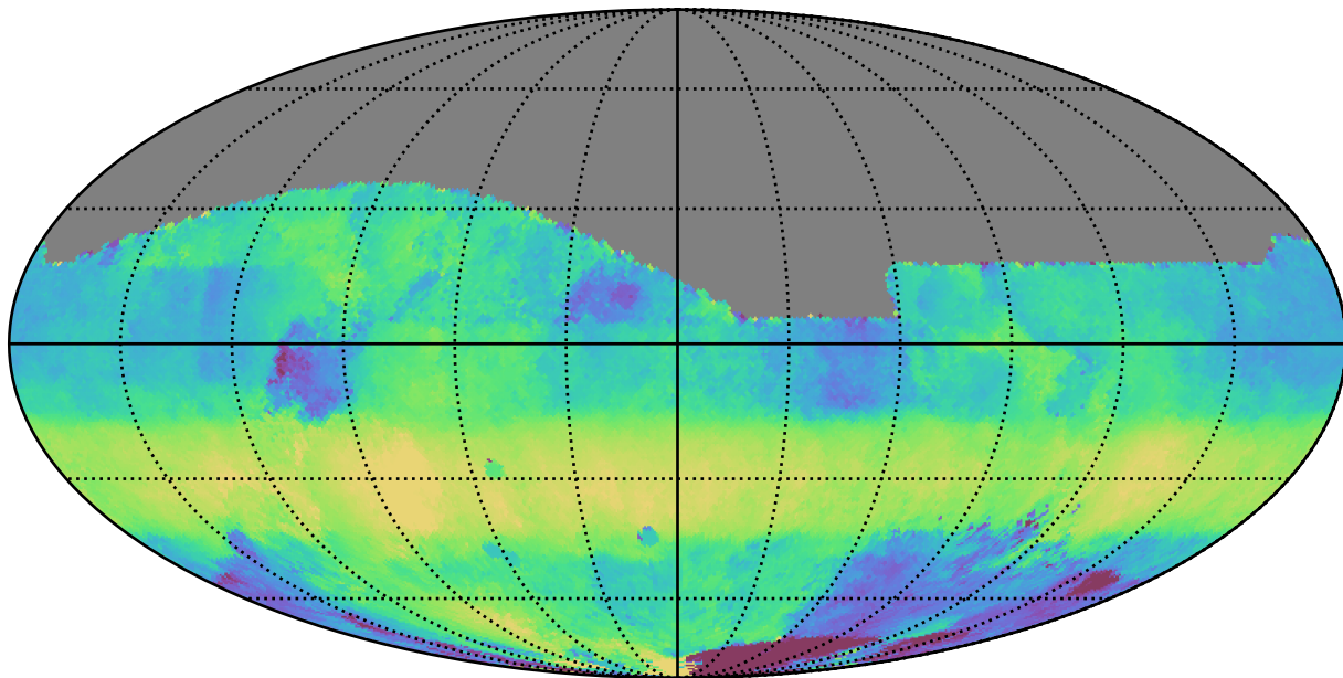
too_elab_heavy_r128_d2_griz_v3.4_10yrs All sky r band: Median HA
