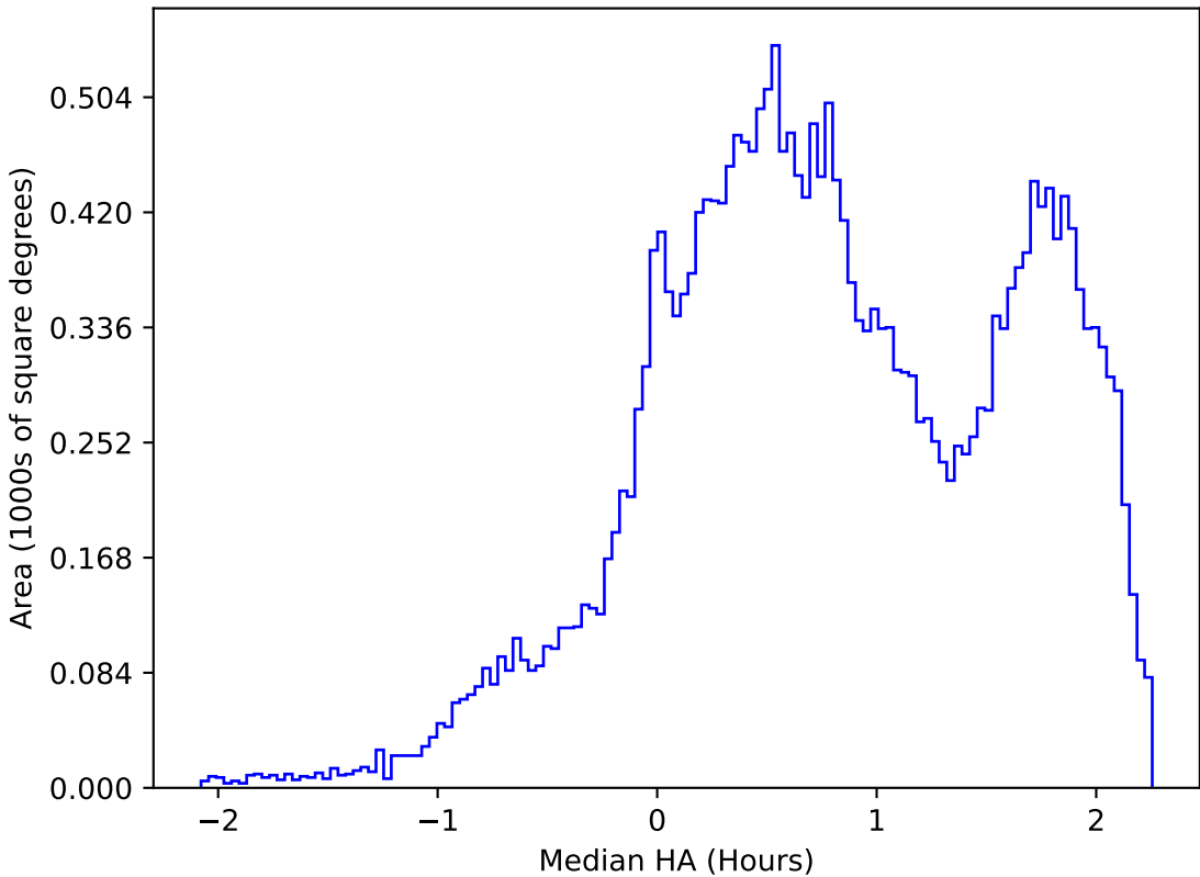
too_elab_heavy_r128_d2_griz_v3.4_10yrs All sky r band: Median HA
