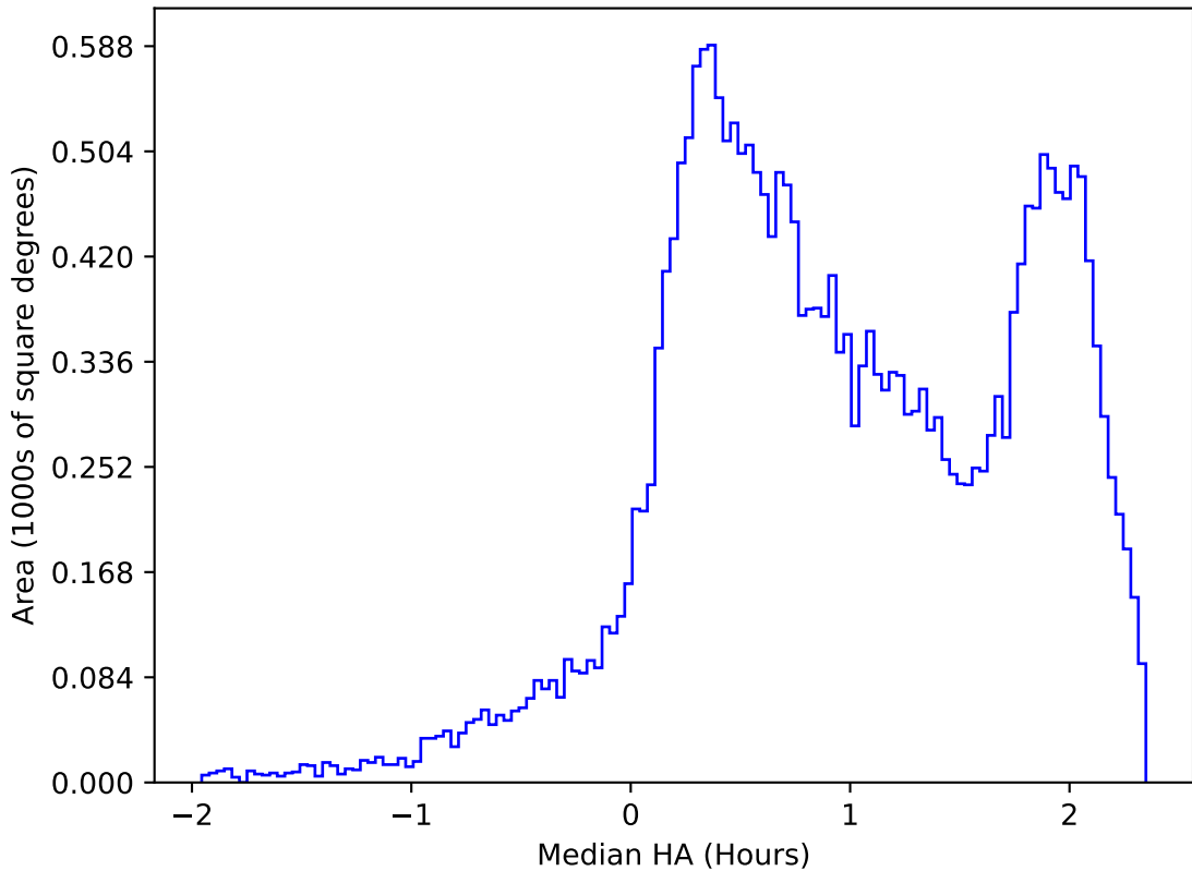
too_elab_heavy_r128_d2_griz_v3.4_10yrs All sky i band: Median HA
