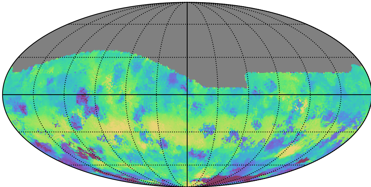
too_elab_heavy_r128_d2_griz_v3.4_10yrs All sky g band: Median HA
