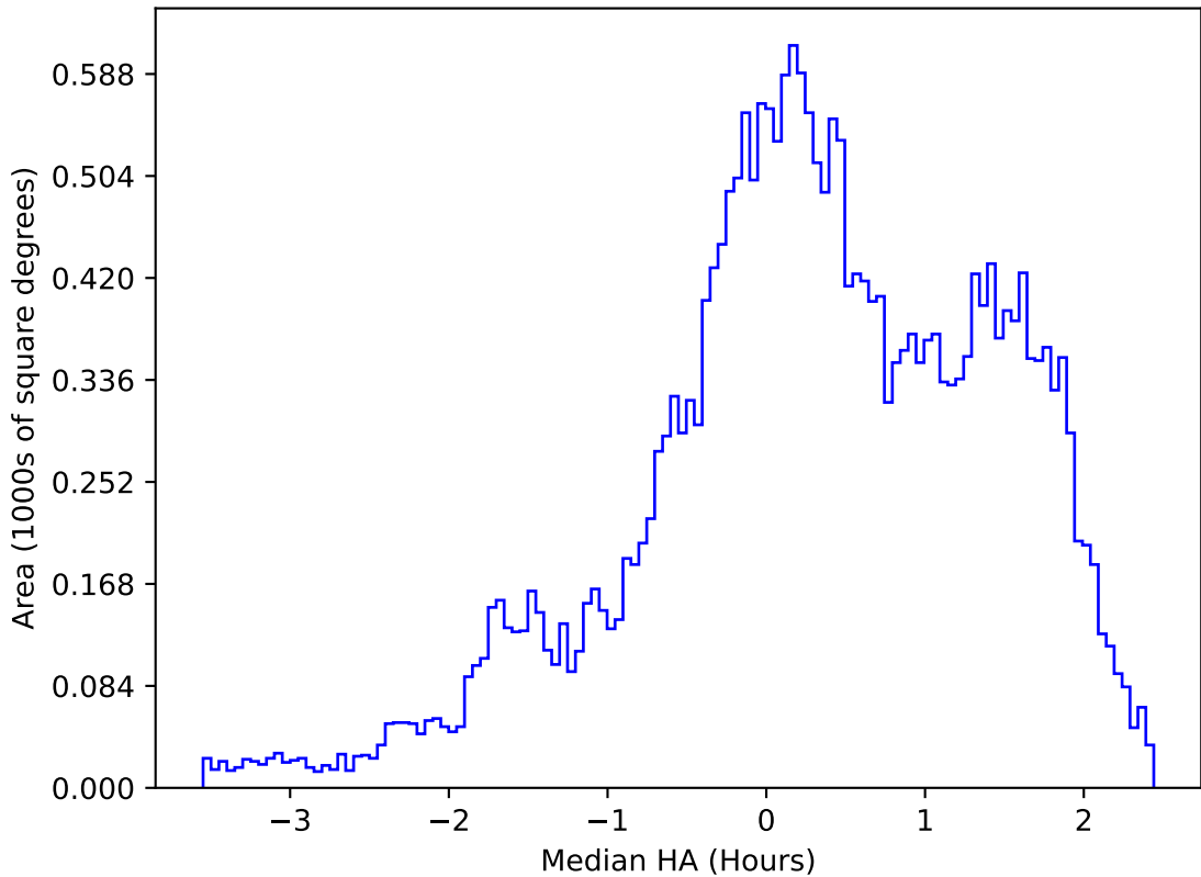
too_elab_heavy_r128_d2_griz_v3.4_10yrs All sky g band: Median HA
