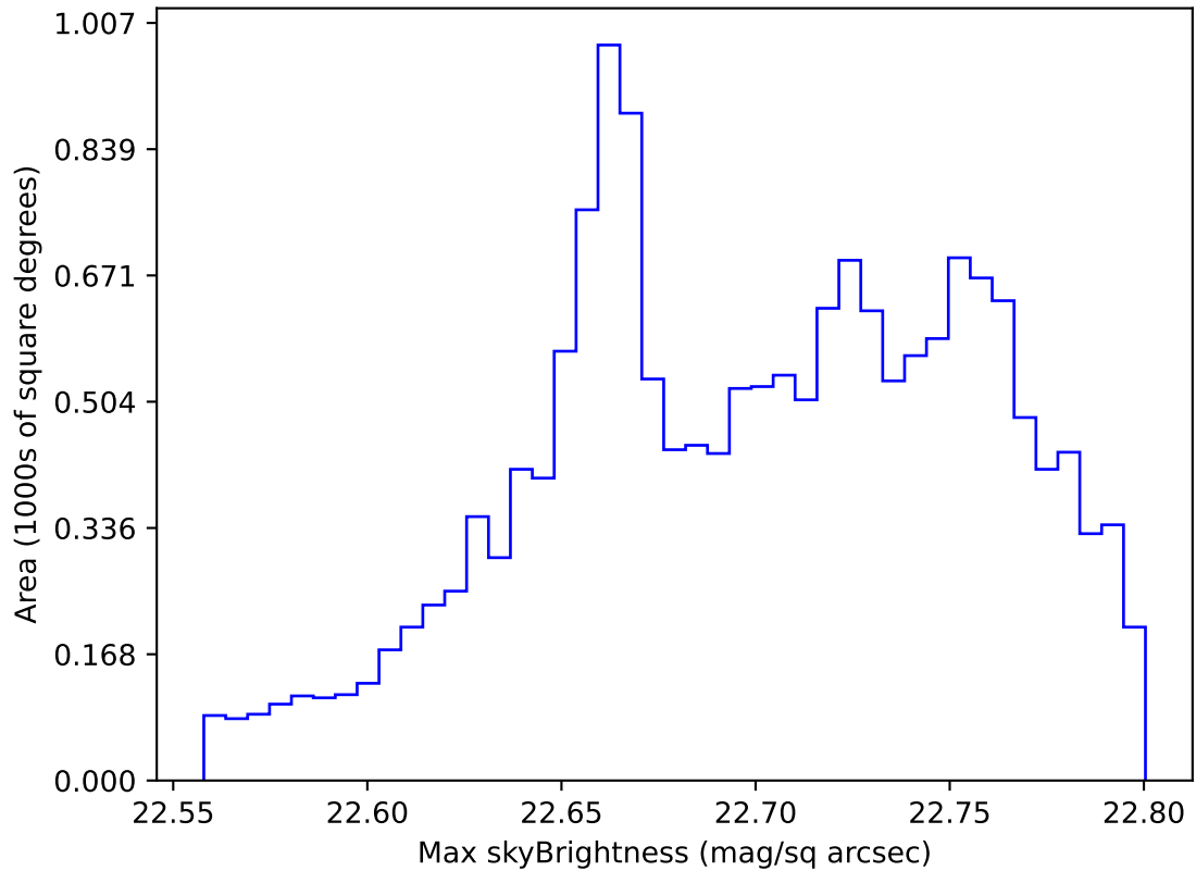
too_elab_heavy_r128_d2_griz_v3.4_10yrs WFD all bands: Max skyBrightness
