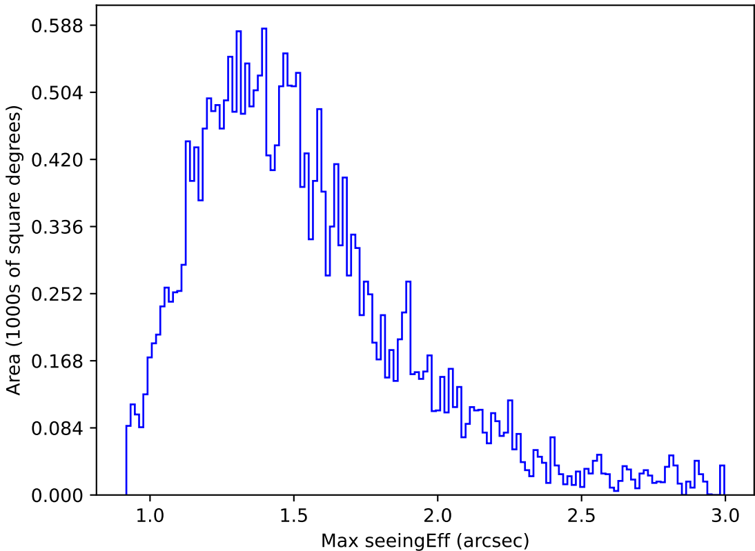
too_elab_heavy_r128_d2_griz_v3.4_10yrs Yr 1 z band: Max seeingEff
