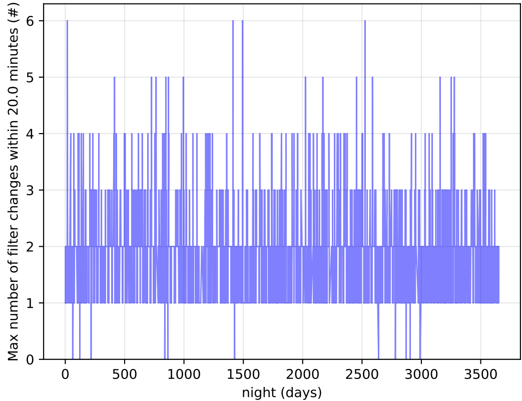
too_elab_heavy_r128_d2_griz_v3.4_10yrs Per Night: Max number of filter changes within 20.0 minutes
