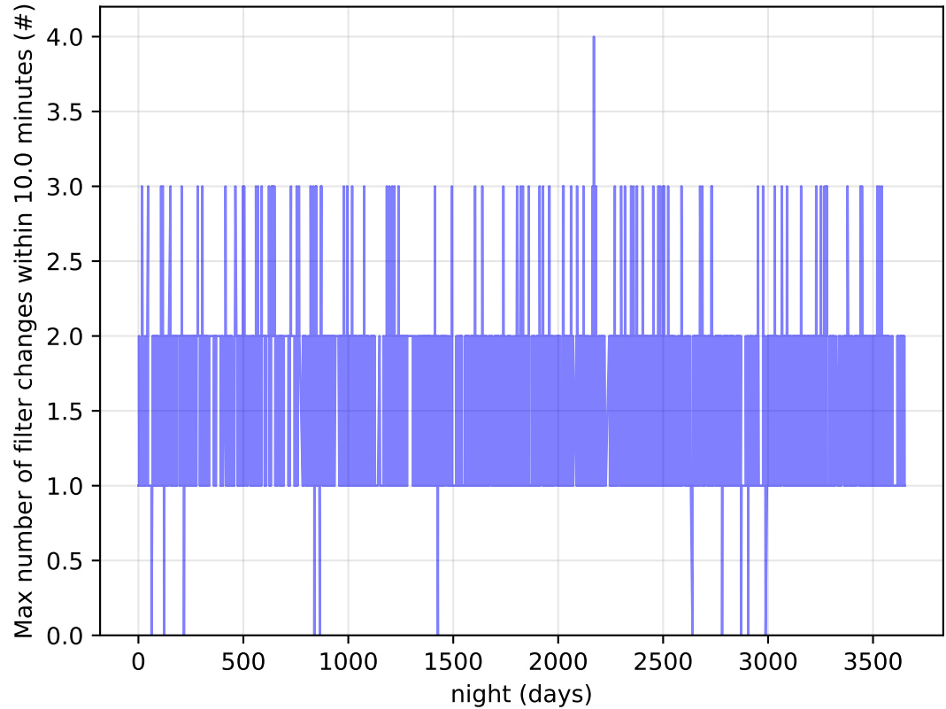
too_elab_heavy_r128_d2_griz_v3.4_10yrs Per Night: Max number of filter changes within 10.0 minutes
