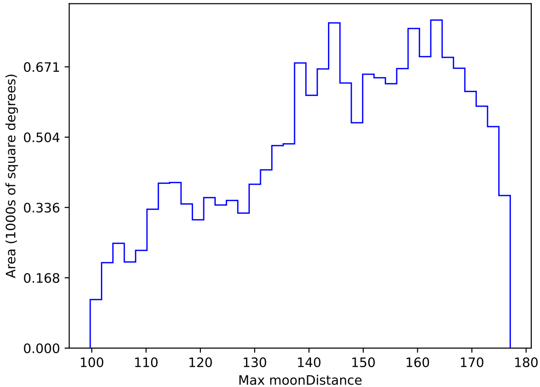
too_elab_heavy_r128_d2_griz_v3.4_10yrs WFD y band: Max moonDistance
