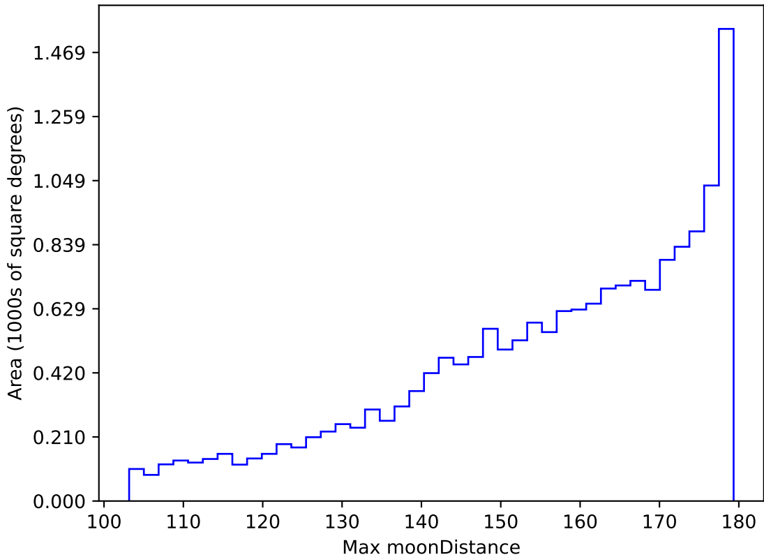
too_elab_heavy_r128_d2_griz_v3.4_10yrs WFD r band: Max moonDistance
