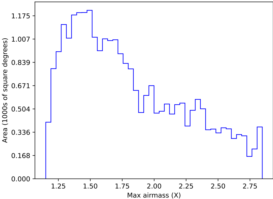
too_elab_heavy_r128_d2_griz_v3.4_10yrs Yr 1 z band: Max airmass
