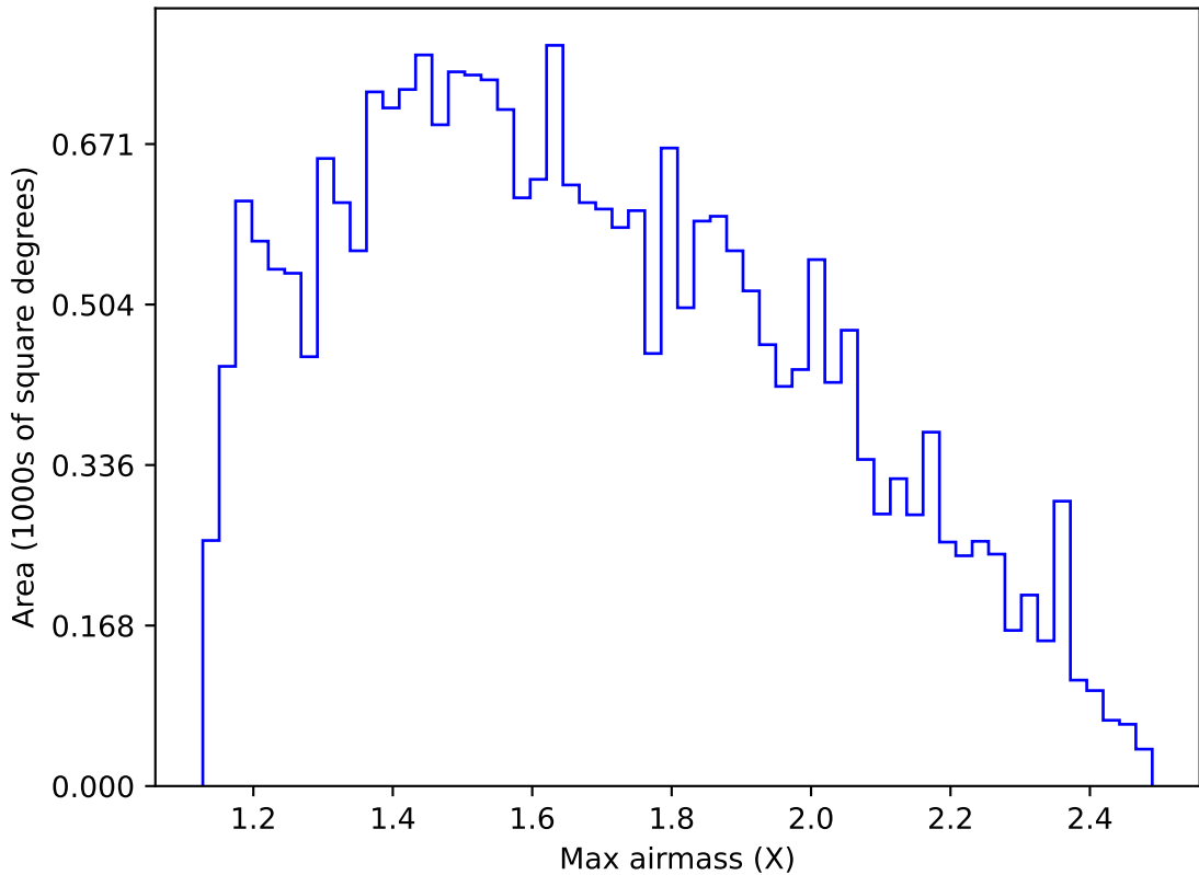
too_elab_heavy_r128_d2_griz_v3.4_10yrs Yr 1 g band: Max airmass
