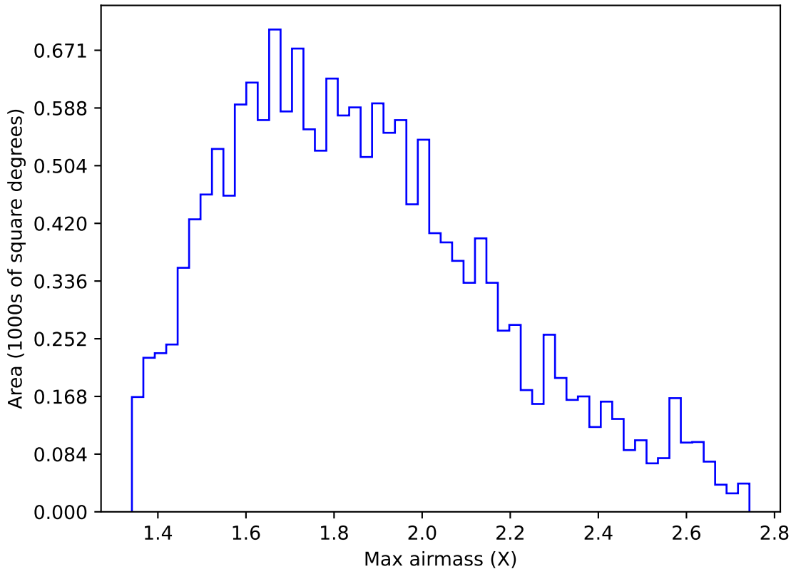
too_elab_heavy_r128_d2_griz_v3.4_10yrs WFD u band: Max airmass
