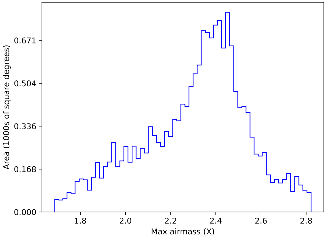
too_elab_heavy_r128_d2_griz_v3.4_10yrs WFD r band: Max airmass
