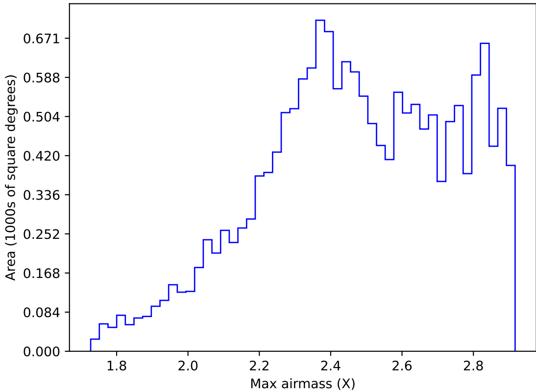
too_elab_heavy_r128_d2_griz_v3.4_10yrs WFD i band: Max airmass
